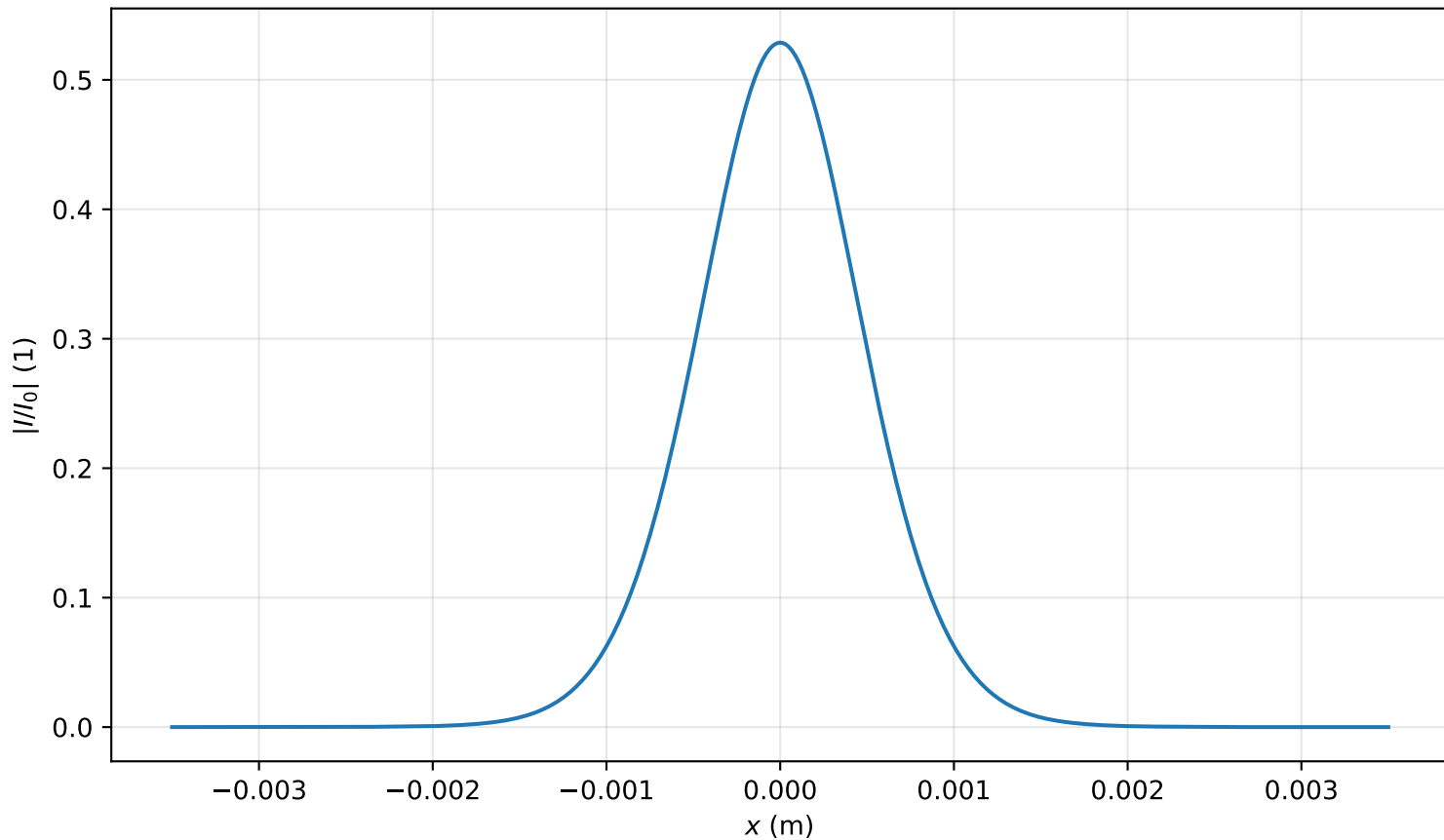
Intensity profile I(x, y = 0, z = 2.786m)/I_0 , P_{in}=0.4P_{cr} , artificial time
